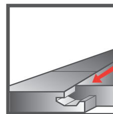
UNICLIC connection
